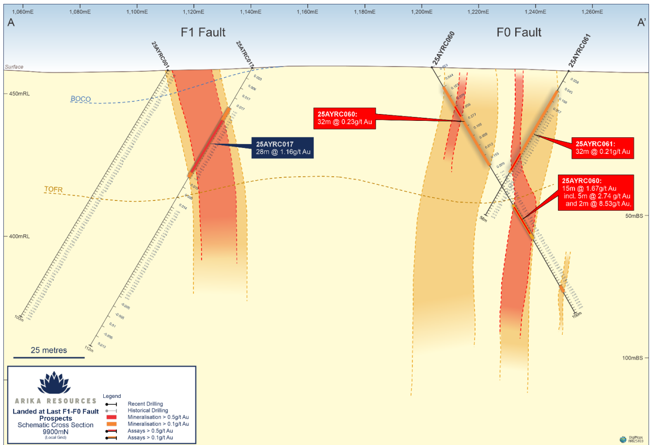
Figure 3: Schematic Cross-Section through the F0 and F1 structures showing recent drilling results and the close proximity of the two structures.
