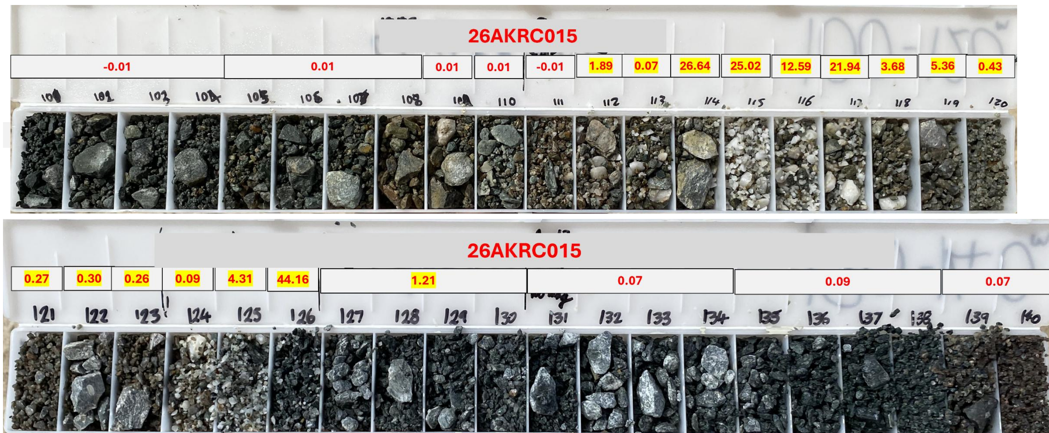
Figure 3: 26AKRC015 Chip tray photo showing high-grade gold mineralisation hosted within sheared and altered mafic volcanics. The 19m interval from 111m downhole depth returned the following:
