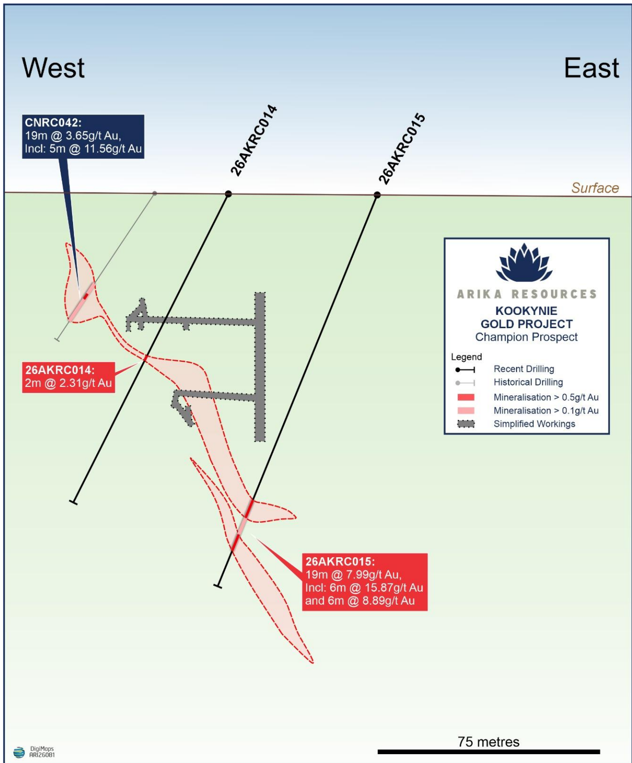
Figure 2: Oblique schematic cross-sectional view. Recent drilling at the historical Champion Gold Mine showing Arika's holes 26AKRC014 and 26AKRC015 in relation to the main shaft and level drives projected south onto this view. The new lode structure identified by holes 26AKRC014 and 26AKRC015 commences south of the underground workings and remains open to the south beyond the plane of the drill section. The interpretation is supported by historical drillhole CNRC042 in this view.
