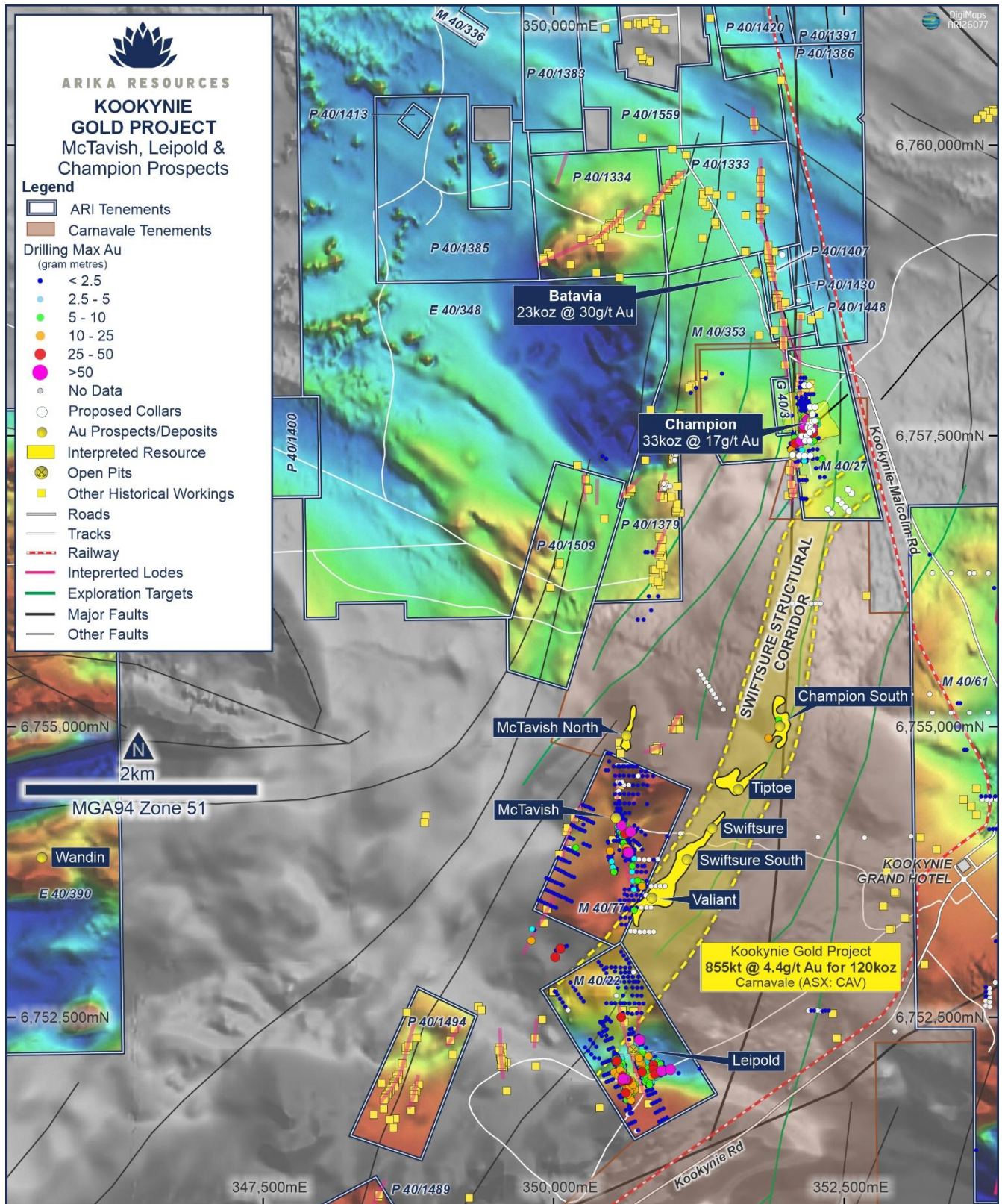
Figure 4: Location plan showing Arika's recent drilling along the Champion-Batavia Trend in relation to the McTavish and Leipold Deposits and Carnavale's Swiftsure Deposits (ASX:CAV)
