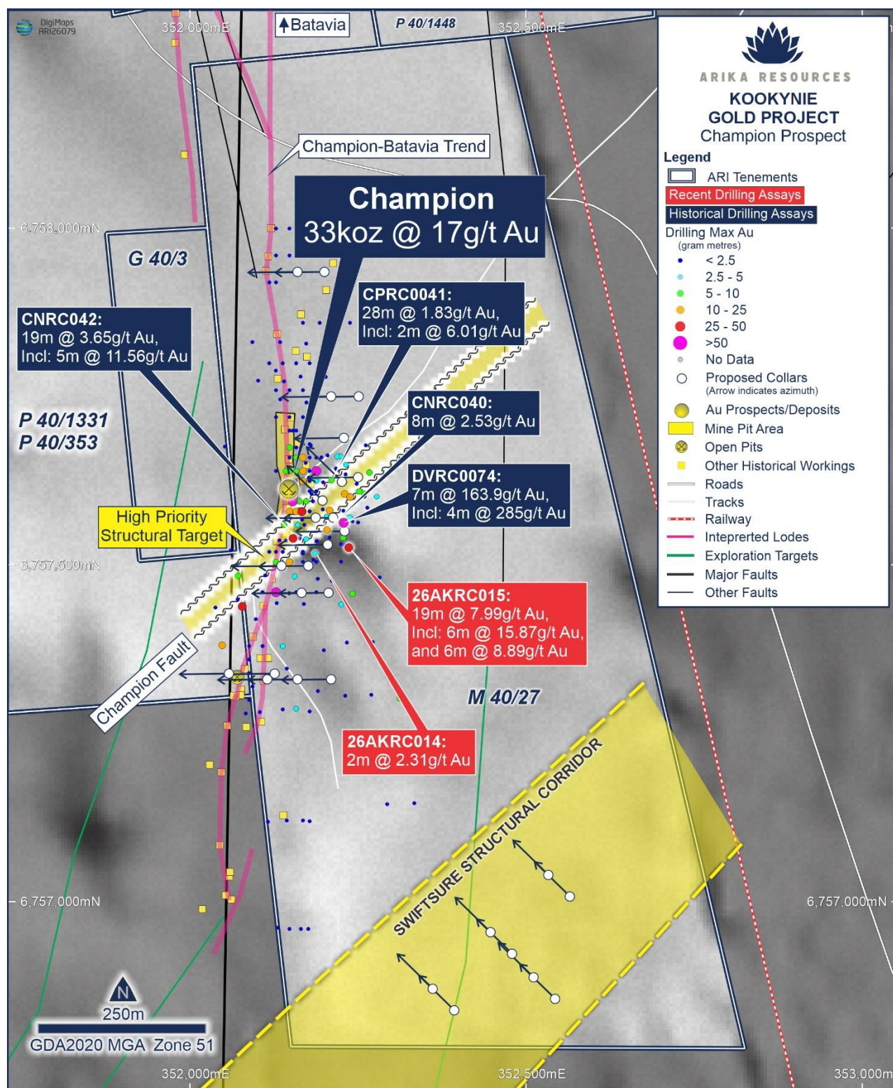
Figure 1: Location plan showing the Champion-Batavia Trend and Arika's recent RC drilling at the Champion Deposit. Note the NE trending 'Swiftsure Structural Corridor' highlighted in yellow with proposed drill traverses.
